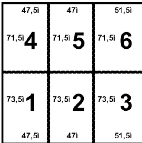
Stall Kit Large 12 ft x 12 ft (Ca. 3,6 x 3,6 meter)
