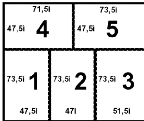
Stall Kit Medium 10 ft x 12 ft (Ca. 3 x 3,6 meter)
